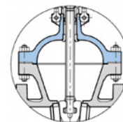
Circular Joint
