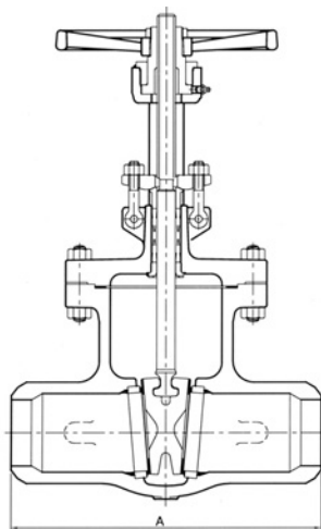
BUTT-WELD END
